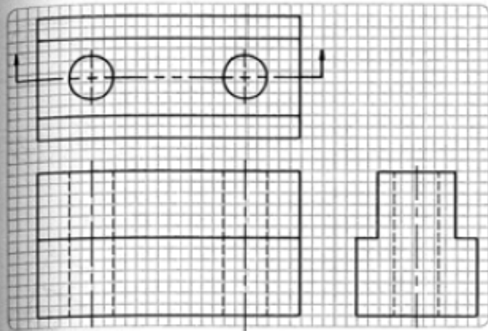
Figure 17.52 Problem 30. Full section.
