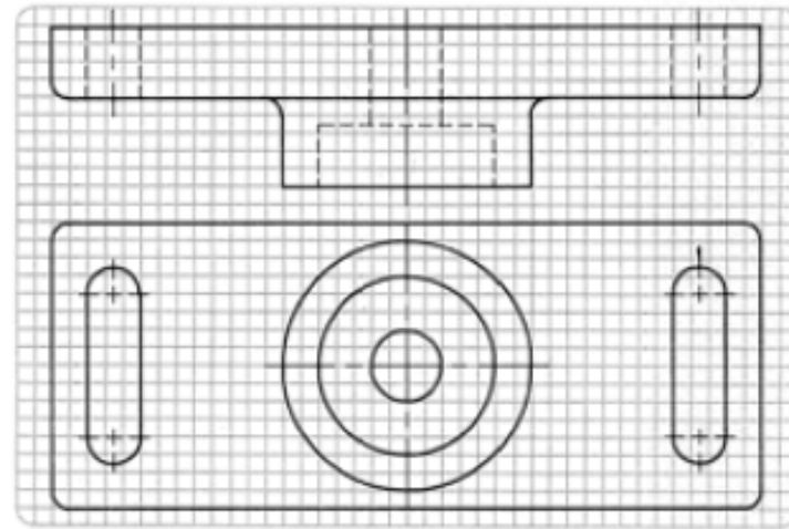
Figure 17.55 Problem 33. Full section.
